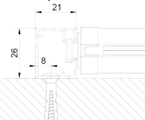
Coulisse pose murale
