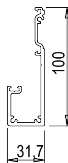
Glass door side beam
