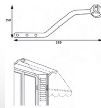
Support persienne
