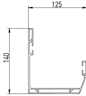
Guide support profile
