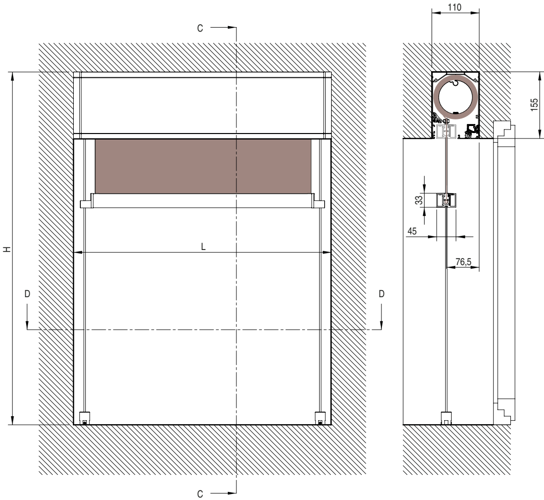
vista posteriore - rear view
