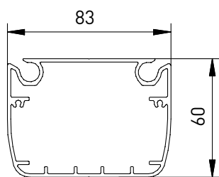
Terminal bar profile
