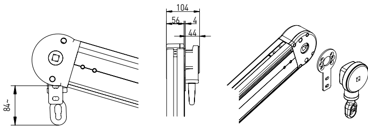
Pulley bracket
