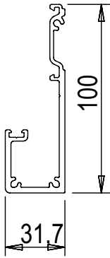
Travesaño lateral porta cristal
