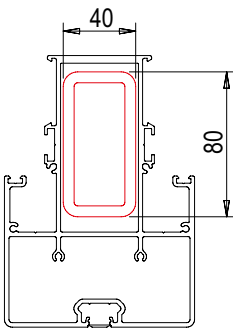
Pillar
