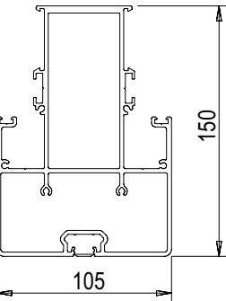
Front beam
