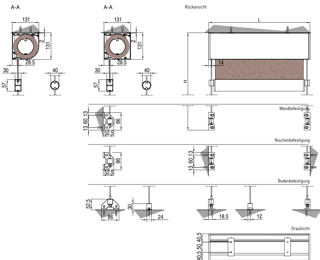
Wandmontage B-B
