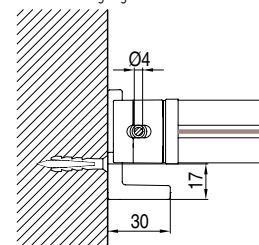
Wandmontage B-B
