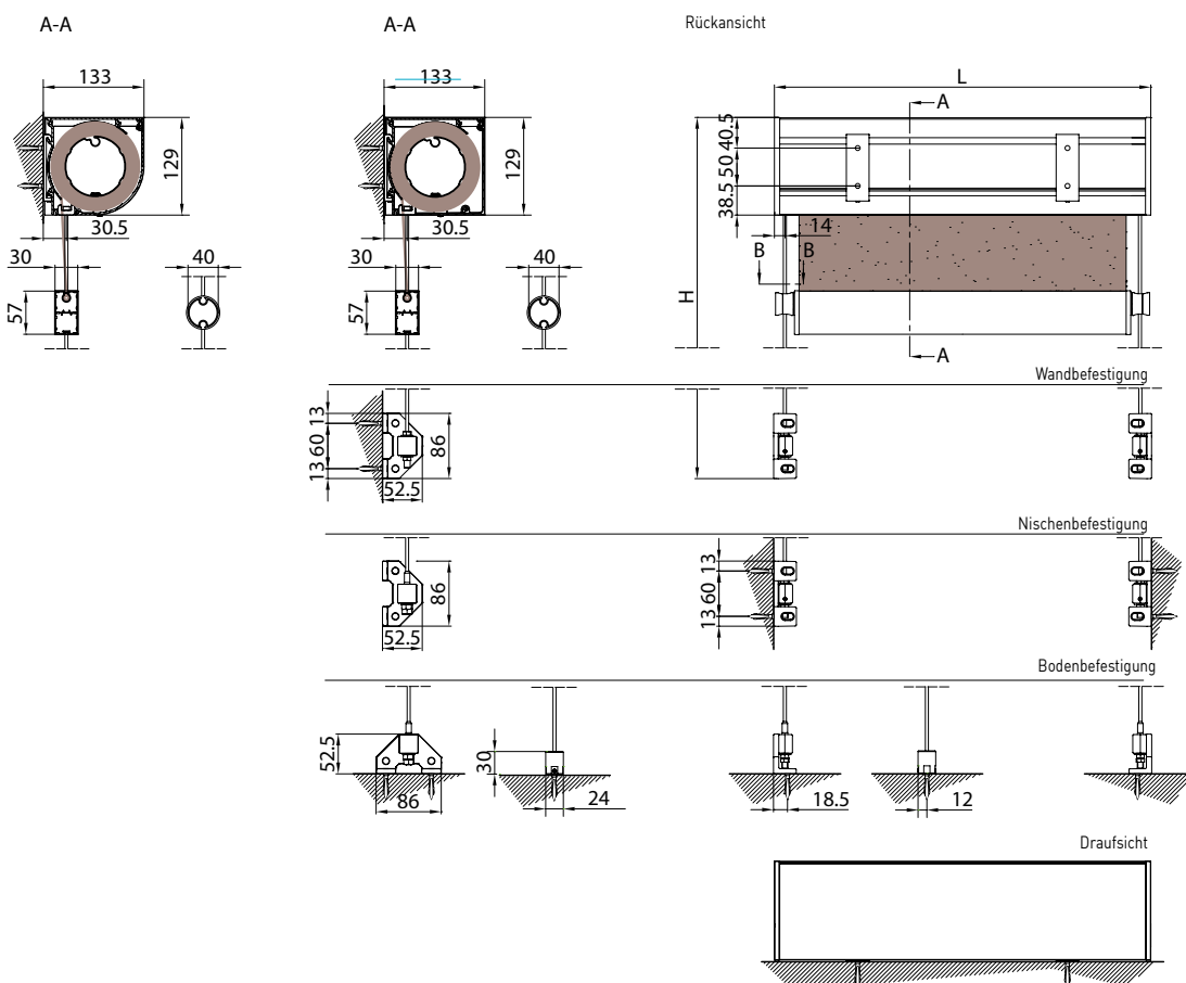
Wandmontage B-B
