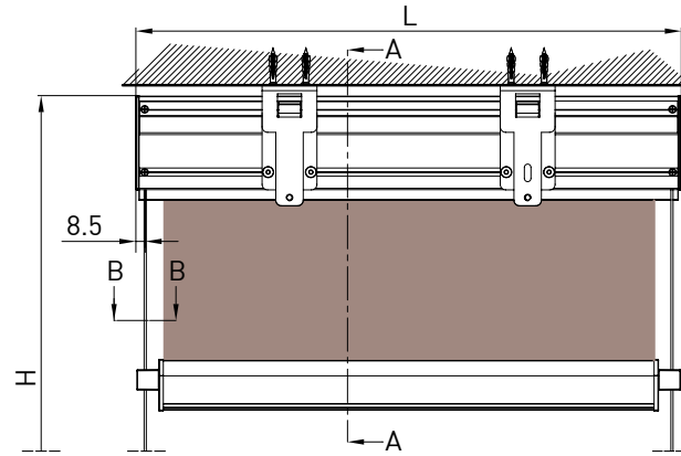
Supporto parete - Wall support - Support au mur - Wandkonsole
