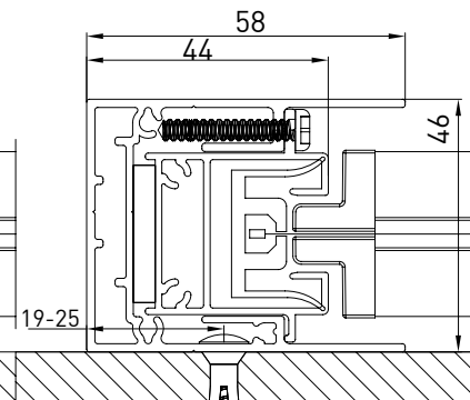
Guida a parete - Wall guide Coulisse façade - Wandführung B-B
