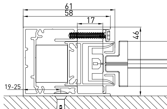
Guida a parete - Wall guide Coulisse façade - Wandführung B-B
