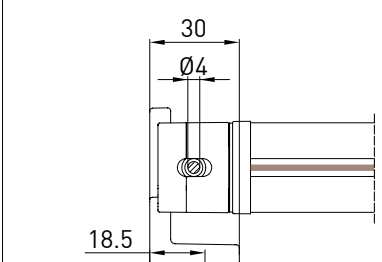
supporto a parete - wall bracket B-B
