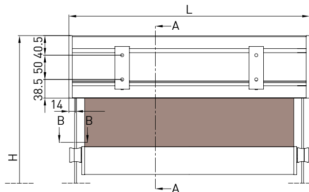
Supporto a parete - Wall support - Support au mur - Wandkonsole
