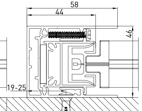
Guida a parete - Wall guide Coulisse façade - Wandführung B-B
