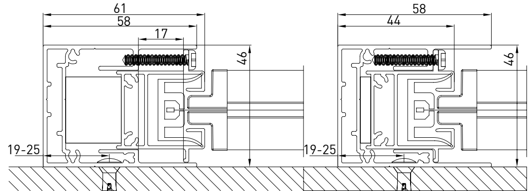
Guida a parete - Wall guide Coulisse façade - Wandführung B-B
