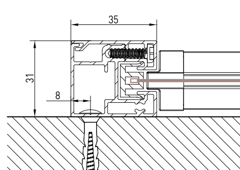
Guida a parete - Wall guide Coulisse façade - Wandführung
