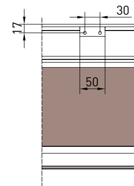
staffa a parete cassetto wall bracket cassette
