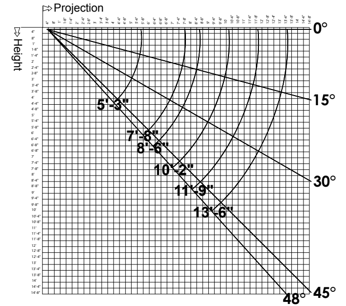
Ceiling covering diagram
