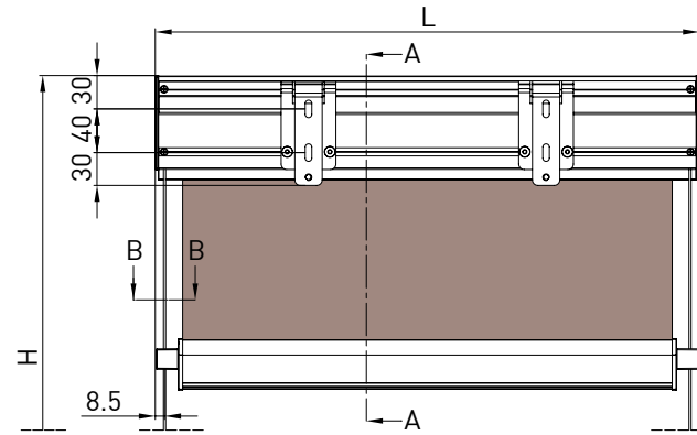
Supporto parete/nicchia - Wall/niche support - Support au mur/niche - Wand/Nischenkonsole
