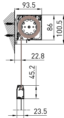
Supporto parete/nicchia - Wall/niche support - Support au mur/niche - Wand/Nischenkonsole
