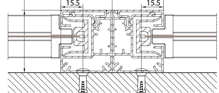
Guida a parete (modulo doppio) - Wall guide (double module) Coulisse façade (module double) - Wandführung (Doppelmodul) C-C
