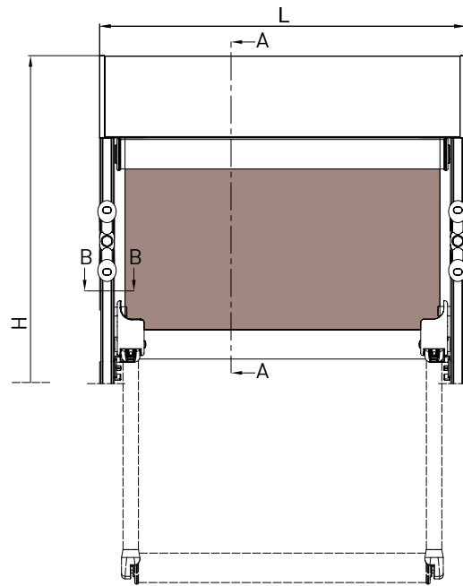
Guida a parete - Wall guide - Coulisse façade - Wandführung
