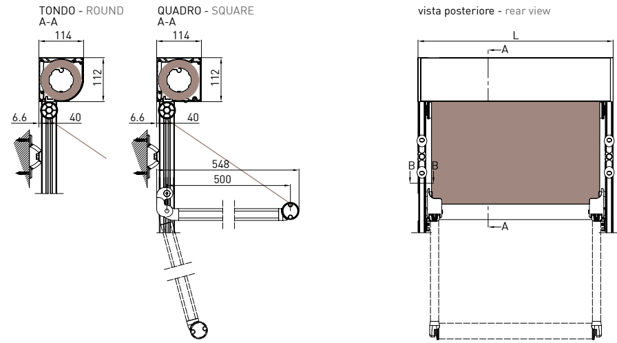
Guida a parete - Wall guide - Coulisse façade - Wandführung
